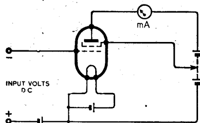
Fig. 1. Basic circuit diagram of a valve voltmeter of which the range of anode current proved too wide.
