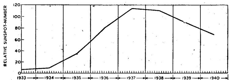
Fig. 1. Yearly means of relative sunspot-numbers for the last seven years.
