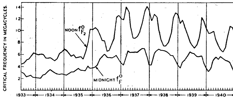
Fig. 2. Monthly average of noon ( f_oF_2 ) and midnight ( f_oF ) critical frequencies at Washington.
