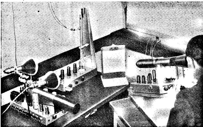
General view of a complete amateur television transmitting station. The operator on the right is viewing the test image on the combined iconoscope and monitoring tube. In the centre is seen the 2\frac{1}{2} metre transmitter while on the left immediately below the two spot light lamps is the receiver.
