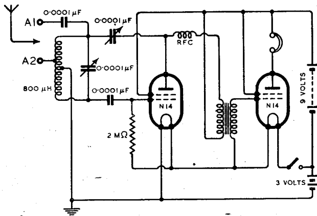
Circuit diagram of a light-weight portable using two 1.4-volt tetrodes as detector and AF amplifier instead of the 2-volt valves originally specified.
