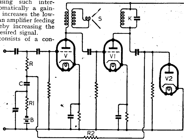
Differential gain-control system
