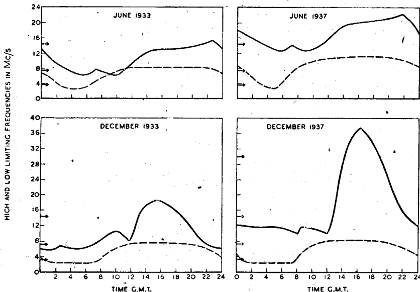
Fig. 3. High and low limiting frequencies for the summer and winter of years at the sunspot minimum and maximum for the transmission path to the U.S.A. by two hops of 3,500 km. each.
