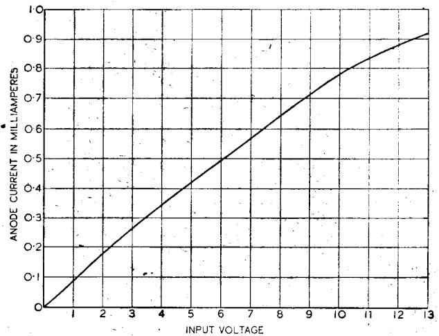
Fig. 4. Calibration curve of the original model of the meter described in this article.
