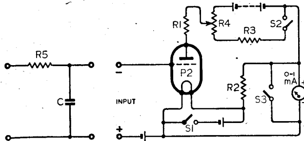
Fig. 3. Final circuit arrangement of the valve voltmeter described.
