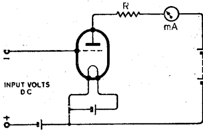
Fig. 2. Triode voltmeter with limiting resistance.
