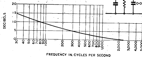
Fig. 2. The correcting circuit used and the resultant curve to be expected.
