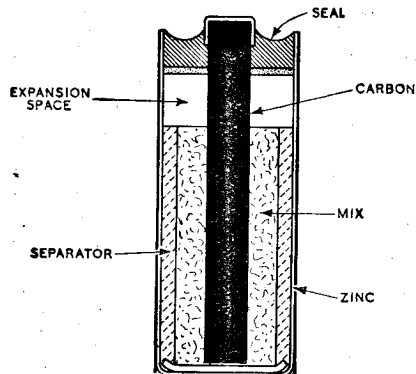
Section of conventional cylindrical-type dry cell.
