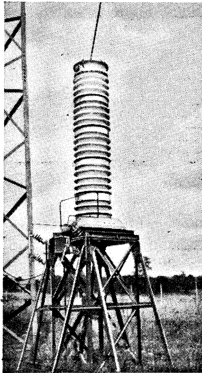
Our contributor admitted last month, when discussing wired wireless broadcasting over the mains, that kilovolts terrified him. Nevertheless, carrier systems are sometimes employed on high-voltage lines; this 0.001 mfd. coupling condenser is used for picking off the carrier current from a 220 kV line.
