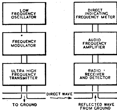
Circuit arrangement for altimeter.
