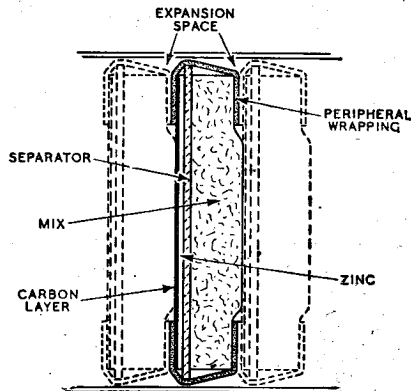
Inter-cell leakage is prevented and expansion permitted by the flexible wrapping of the latest flat-type dry cell.
