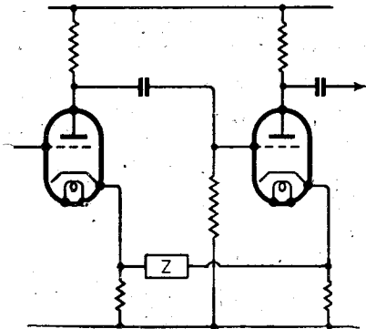
Cathode-impedance frequency control.
