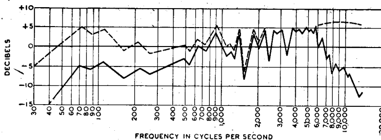
Fig. 1. The heavy line shows the response curve of the writer's loud speaker before correction, and the dotted line the approximate curve after correction. The decibel scale has been opened out to give a clearer effect of the result obtained.
